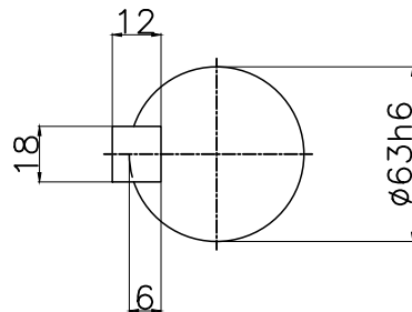
OUTPUT SHAFT
